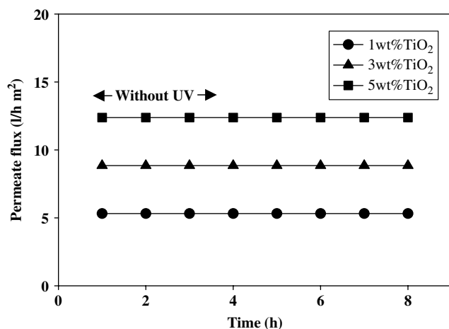
Figure 6. The permeate flux vs reaction time of polyacrylonitrile membranes at various percentages of TiO 2 and pH 3.
