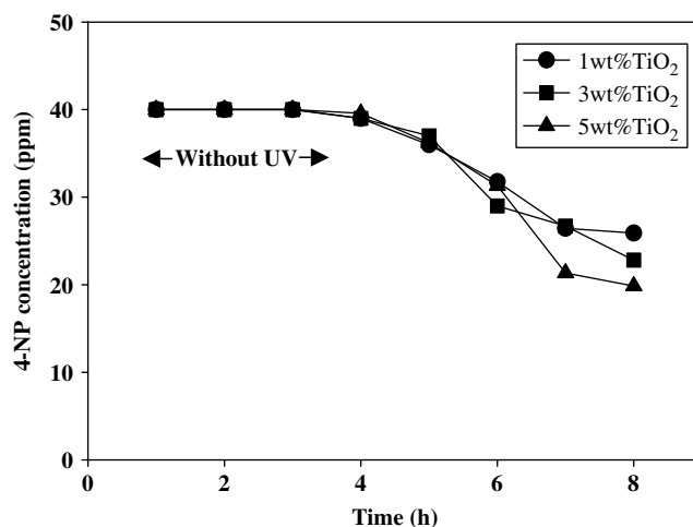
Figure 7. The degradation of 4-NP with the reaction time of polyacrylonitrile membranes at various percentages of TiO 2 and pH 3.
