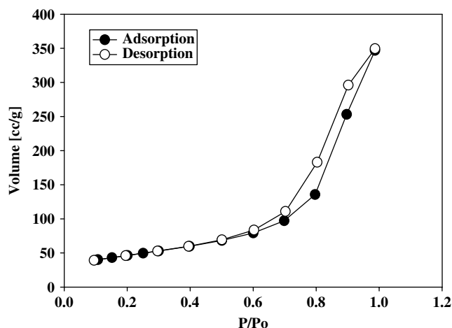
Figure 3. Nitrogen adsorption–desorption isotherm for the prepared mesoporous titania calcined at 600 °C.
