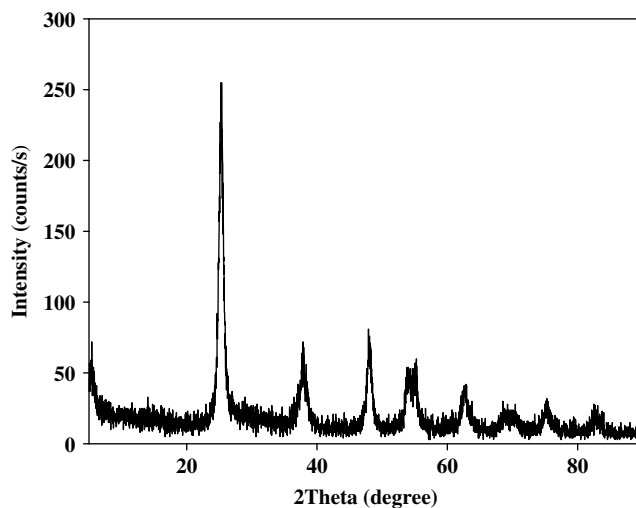
Figure 2. XRD pattern of the anatase phase of the prepared TiO 2 catalyst after calcinations of the precursor at 600 °C for 2 h.
