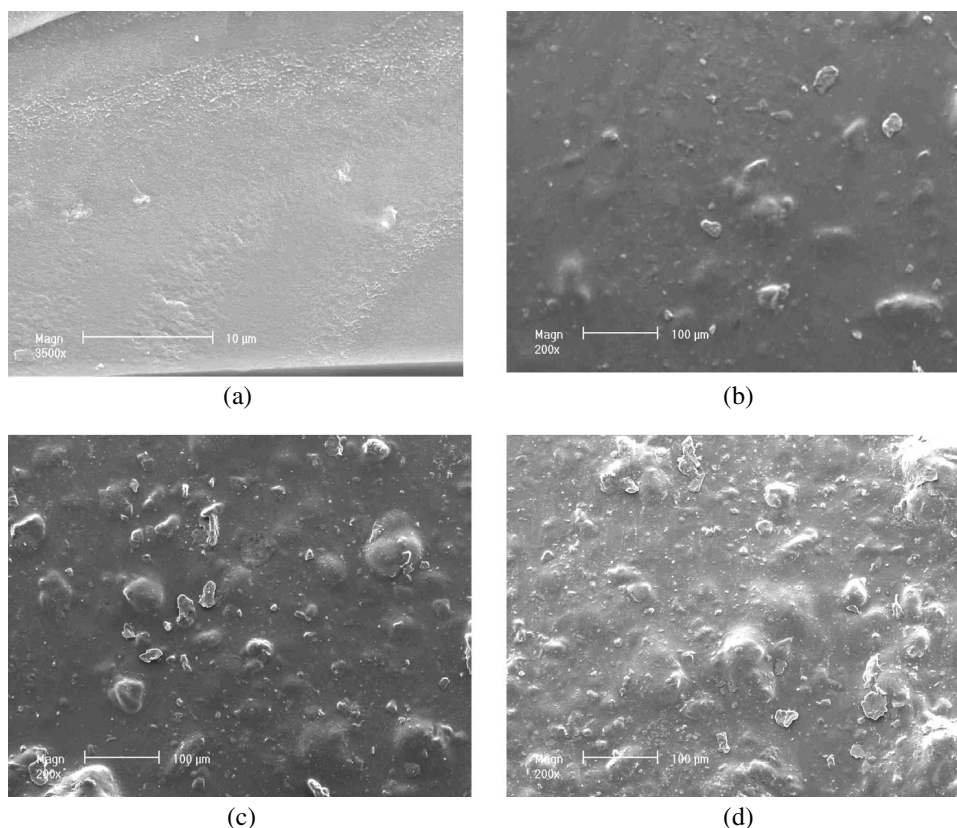
Figure 4. SEM micrographs of mixed matrix membranes using (a) polyacrylonitrile (PAN), (b) PAN + 1 wt% TiO 2 , (c) PAN + 3 wt% TiO 2 and (d) PAN + 5 wt% TiO 2 .
