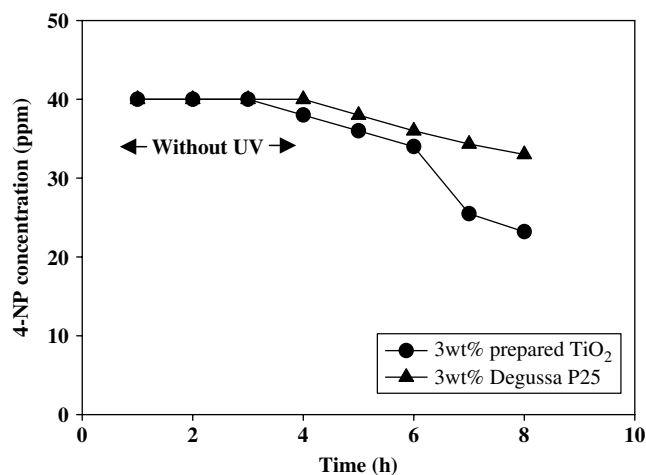
Figure 8. Effect of TiO 2 type mixed in the polyacrylonitrile membrane on the degradation of 4-NP.
